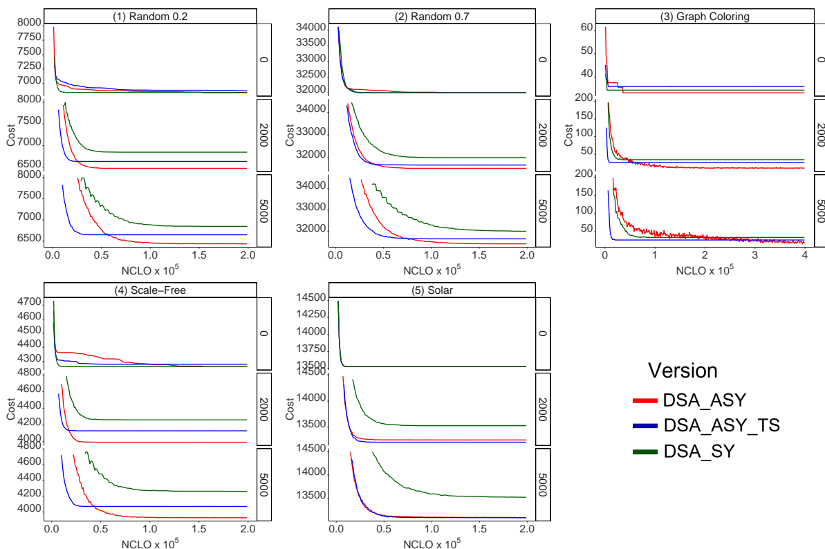
Figure 2: Costs of solutions for both synchronous and asynchronous DSA with different lengths of message delays sampled from a uniform distribution (Subgraphs 1-4) and Poisson distribution (Subgraph 5). Figure 14 in the appendix shows the corresponding color-blind friendly figure.
