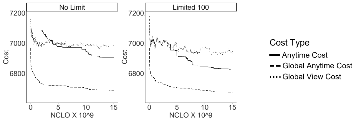
Figure 22: Global view solution cost, global view anytime cost and the anytime cost reported by AAM, of DSA_SDP solving sparse uniform random problems, without memory limitation (left) and with memory limitation to 100 contexts per agent (right). Message delays were sampled from a uniform distribution.
