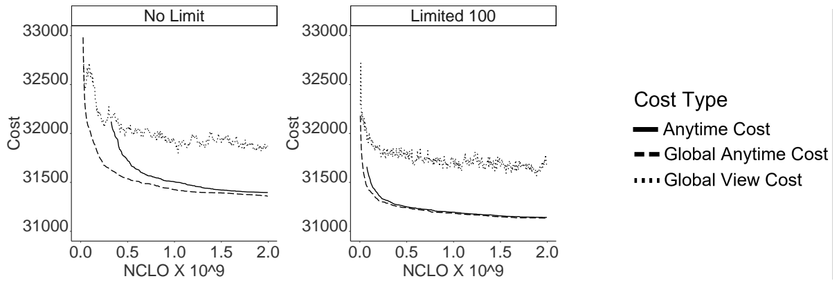
Figure 24: Global view solution cost, global view anytime cost and the anytime cost reported by AAM, of DSA_SDP solving dense uniform random problems, without memory limitation (left) and with memory limitation to 100 contexts per agent (right). Message delays were sampled from a Uniform distribution.
