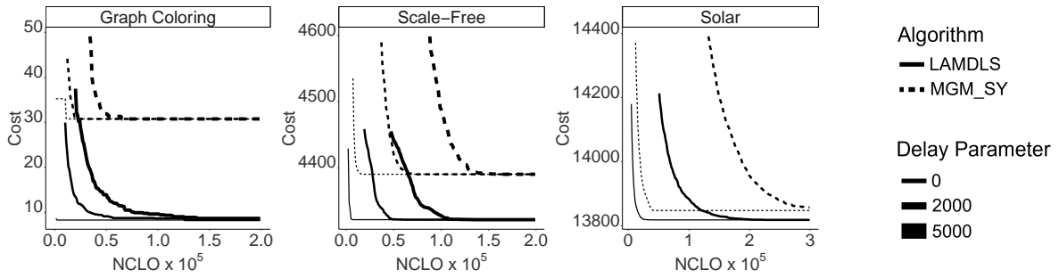
Figure 20: Solution quality of LAMDLS and synchronous MGM, as a function of NCLOs, solving Graph Coloring (left), Scale-Free Networks (middle) and Solar System (right) problems.
