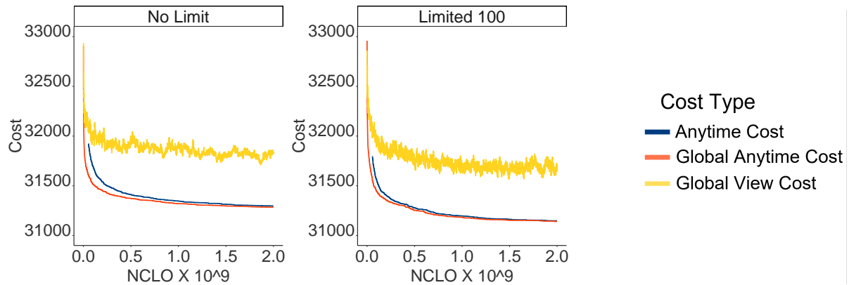
Figure 12: Global view solution cost, global view anytime cost and the anytime cost reported by AAM, of DSA_SDP solving dense uniform random problems, without memory limitation (left) and with memory limitation to 100 contexts per agent (right). Messages were delivered with no delay. Figure 23 in the appendix shows the corresponding color-blind friendly figure.
