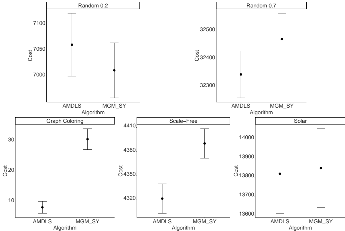
Figure 9: Average solution quality with standard error bars of LAMDLS and synchronous MGM at termination.
