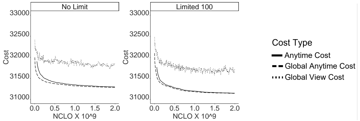
Figure 23: Global view solution cost, global view anytime cost and the anytime cost reported by AAM, of DSA_SDP solving dense uniform random problems, without memory limitation (left) and with memory limitation to 100 contexts per agent (right). Messages were delivered with no delay.
