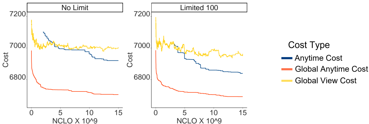
Figure 11: Global view solution cost, global view anytime cost and the anytime cost reported by AAM, of DSA_SDP solving sparse uniform random problems, without memory limitation (left) and with memory limitation to 100 contexts per agent (right). Message delays were sampled from a uniform distribution. Figure 22 in the appendix shows the corresponding color-blind friendly figure.
