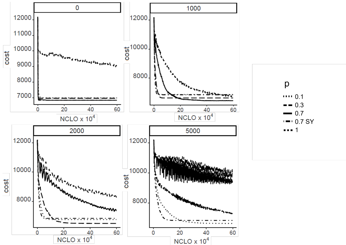
Figure 16: Solution cost of asynchronous DSA without timestamp, using different p values, when solving sparse uniform random problems, with delays sampled from a Poisson distribution.
