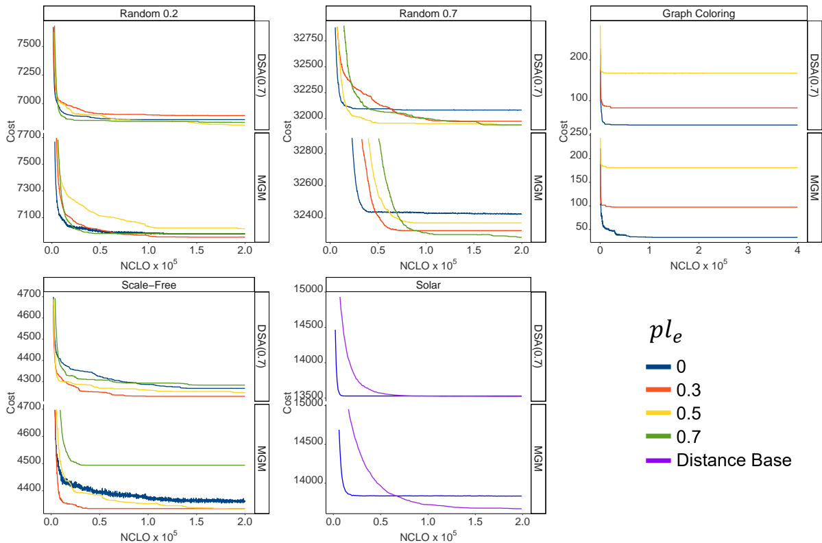
Figure 6: Solution quality of Asynchronous DSA and Asynchronous MGM, as a function of NCLOs. Experiments including various probabilities for message loss. Figure 18 in the appendix shows the corresponding color-blind friendly figure.
