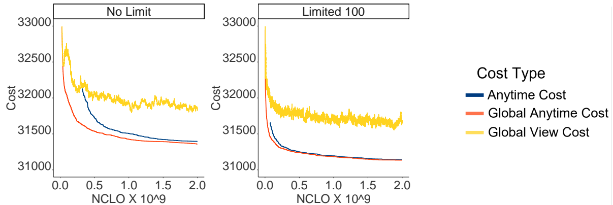
Figure 13: Global view solution cost, global view anytime cost and the anytime cost reported by AAM, of DSA_SDP solving dense uniform random problems, without memory limitation (left) and with memory limitation to 100 contexts per agent (right). Message delays were sampled from a Uniform distribution. Figure 24 in the appendix shows the corresponding color-blind friendly figure.
