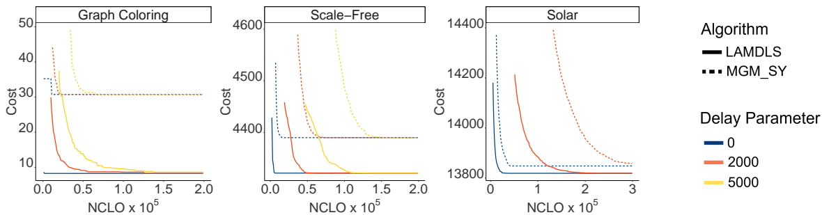
Figure 8: Solution quality of LAMDLS and synchronous MGM, as a function of NCLOs, solving Graph Coloring (left), Scale-Free Networks (middle) and Solar System (right) problems. Figure 20 in the appendix shows the corresponding color-blind friendly figure.
