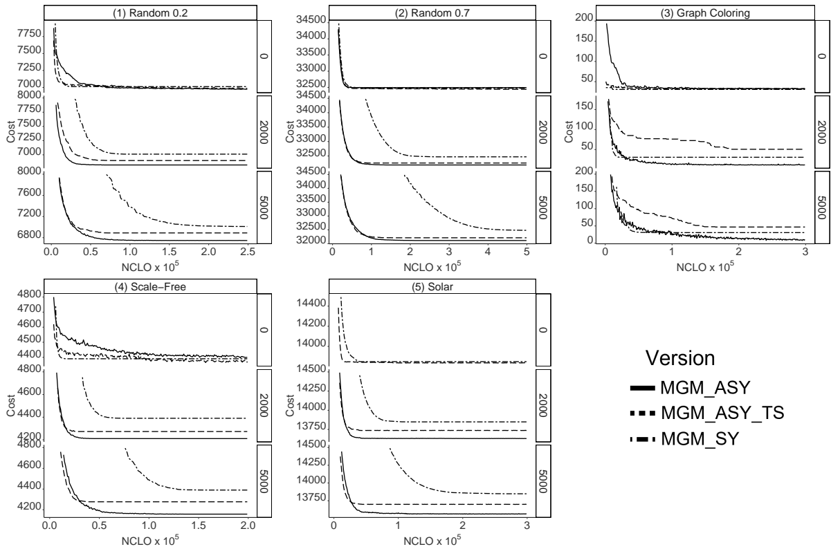
Figure 15: Costs of solutions for both synchronous and asynchronous MGM with different lengths of message delays sampled from a uniform distribution (Subgraphs 1-4) and Poisson distribution (Subgraph 5).
