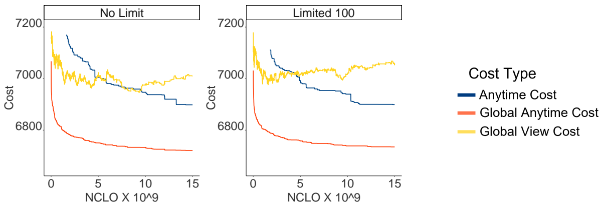
Figure 10: Global view solution cost, global view anytime cost and the anytime cost reported by AAM, of DSA_SDP solving sparse uniform random problems, without memory limitation (left) and with memory limitation to 100 contexts per agent (right). Messages were delivered with no delay. Figure 21 in the appendix shows the corresponding color-blind friendly figure.
