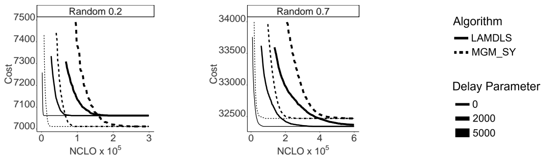
Figure 19: Solution quality of LAMDLS and synchronous MGM, as a function of NCLOs, solving sparse (left) and dense (right) uniform random problems.
