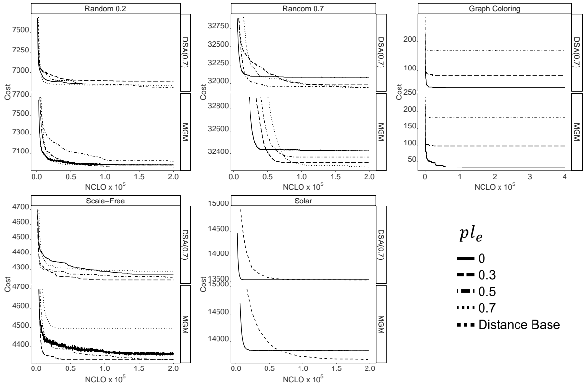
Figure 18: Solution quality of Asynchronous DSA and Asynchronous MGM, as a function of NCLOs. Experiments including various probabilities for message loss.
