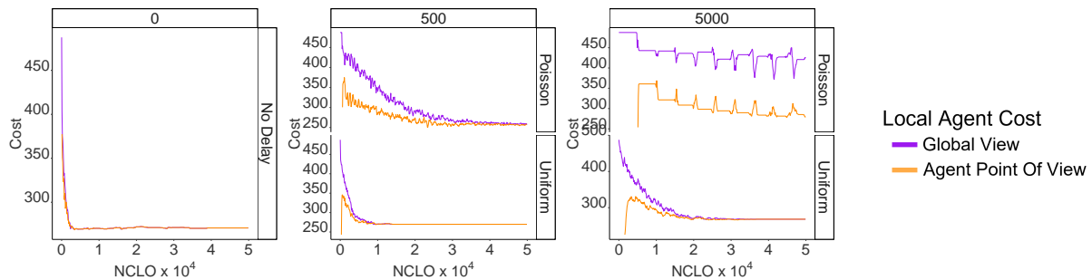
Figure 5: Local costs of a single agent performing asynchronous DSA, solving sparse uniform random problems. Figure 17 in the appendix shows the corresponding color-blind friendly figure.
