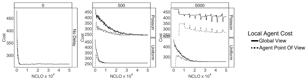
Figure 17: Local costs of a single agent performing asynchronous DSA, solving sparse uniform random problems.
