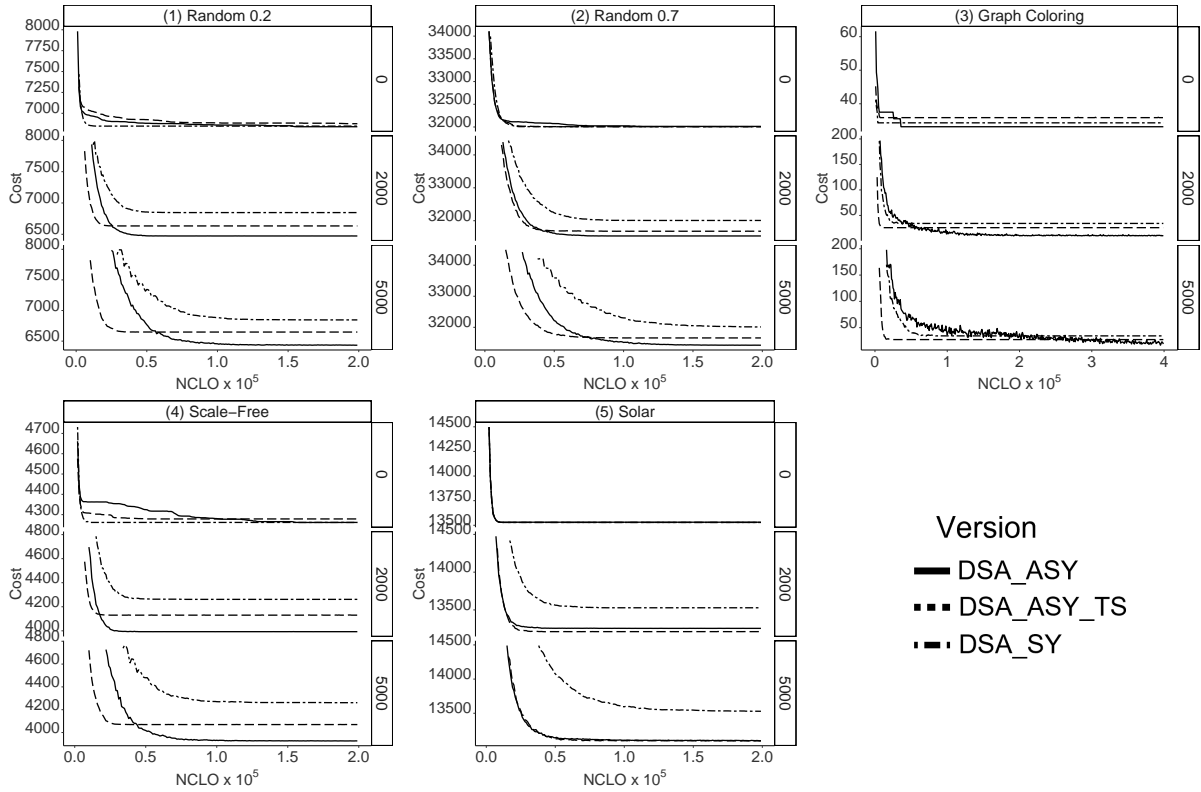
Figure 14: Costs of solutions for both synchronous and asynchronous DSA with different lengths of message delays sampled from a uniform distribution (Subgraphs 1-4) and Poisson distribution (Subgraph 5).
