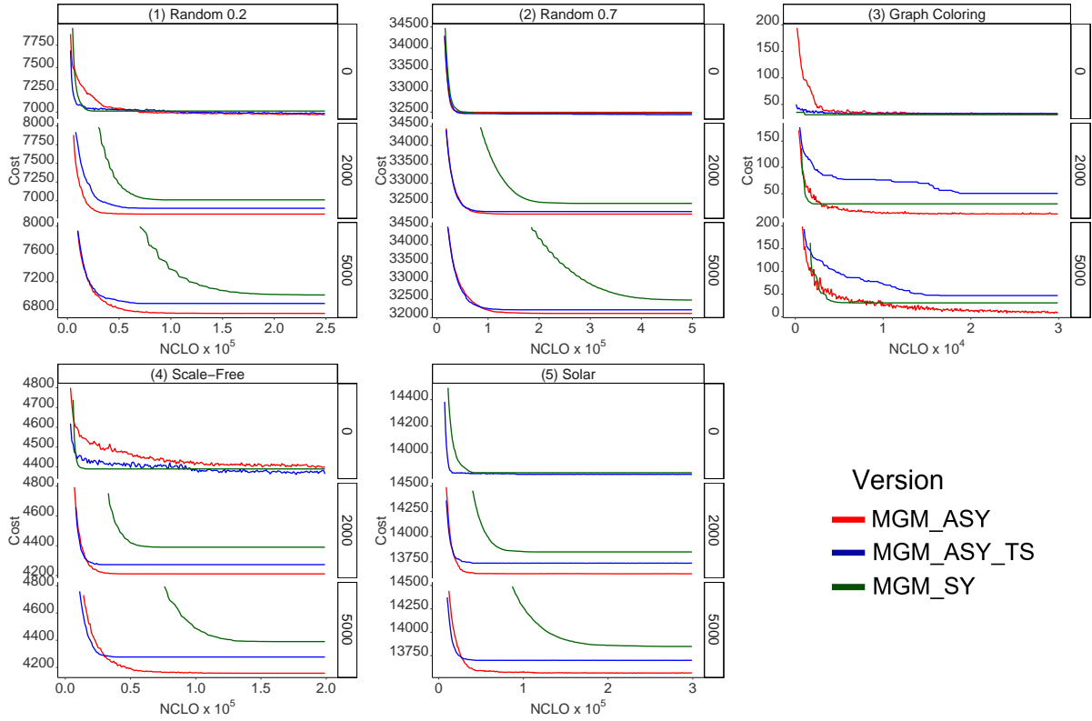
Figure 3: Costs of solutions for both synchronous and asynchronous MGM with different lengths of message delays sampled from a uniform distribution (Subgraphs 1-4) and Poisson distribution (Subgraph 5). Figure 15 in the appendix shows the corresponding color-blind friendly figure.
