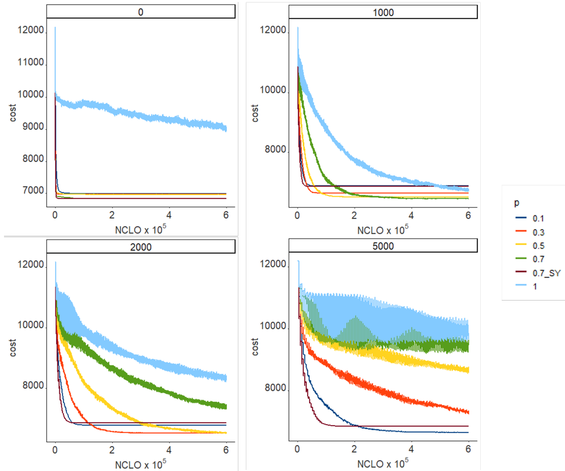
Figure 4: Solution cost of asynchronous DSA without timestamp, using different p values, when solving sparse uniform random problems, with delays sampled from a Poisson distribution. Figure 16 in the appendix shows the corresponding color-blind friendly figure.
