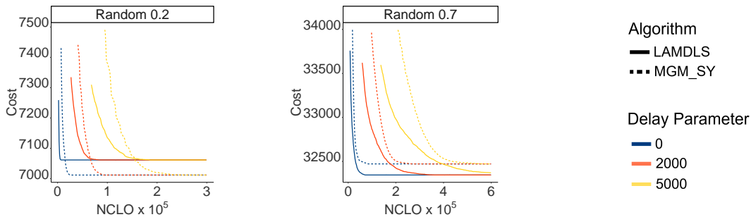
Figure 7: Solution quality of LAMDLS and synchronous MGM, as a function of NCLOs, solving sparse (left) and dense (right) uniform random problems. Figure 19 in the appendix shows the corresponding color-blind friendly figure.
