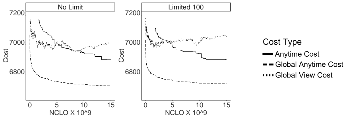
Figure 21: Global view solution cost, global view anytime cost and the anytime cost reported by AAM, of DSA_SDP solving sparse uniform random problems, without memory limitation (left) and with memory limitation to 100 contexts per agent (right). Messages were delivered with no delay.
