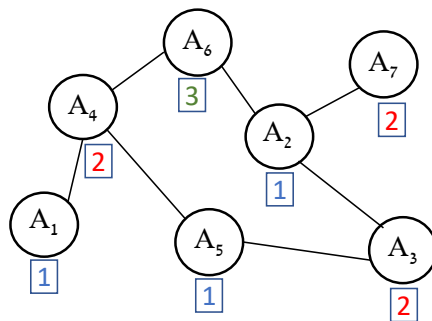
Figure 1: A numerical graph color partition.
